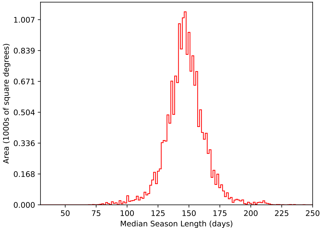
too_elab_r64_d3_griz_v3.4_10yrs WFD i band: Median Season Length
