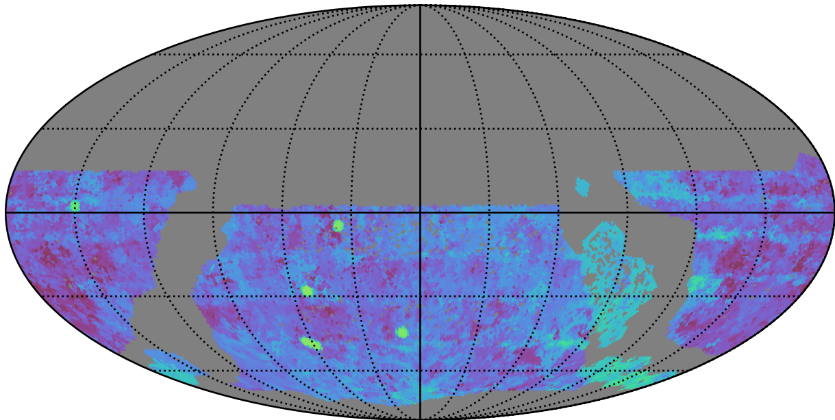
too_elab_r64_d3_griz_v3.4_10yrs WFD g band: Median Season Length
