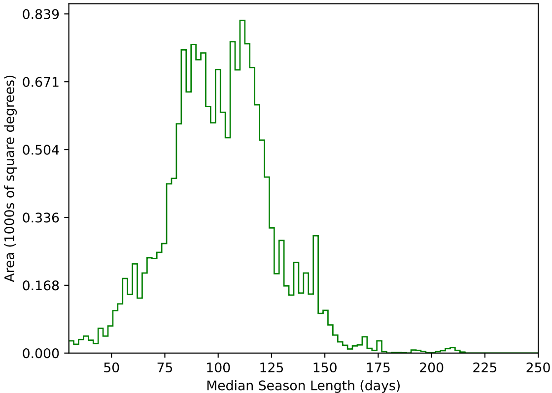
too_elab_r64_d3_griz_v3.4_10yrs WFD g band: Median Season Length
