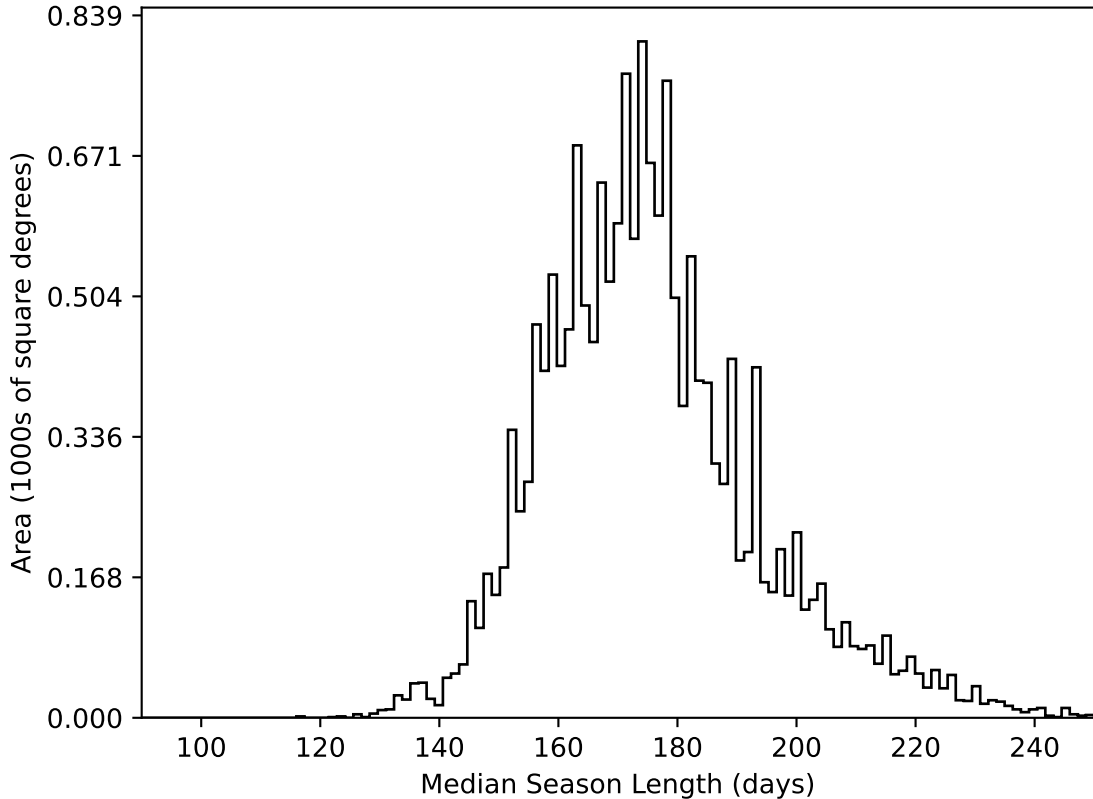
too_elab_r64_d3_griz_v3.4_10yrs WFD all bands: Median Season Length
