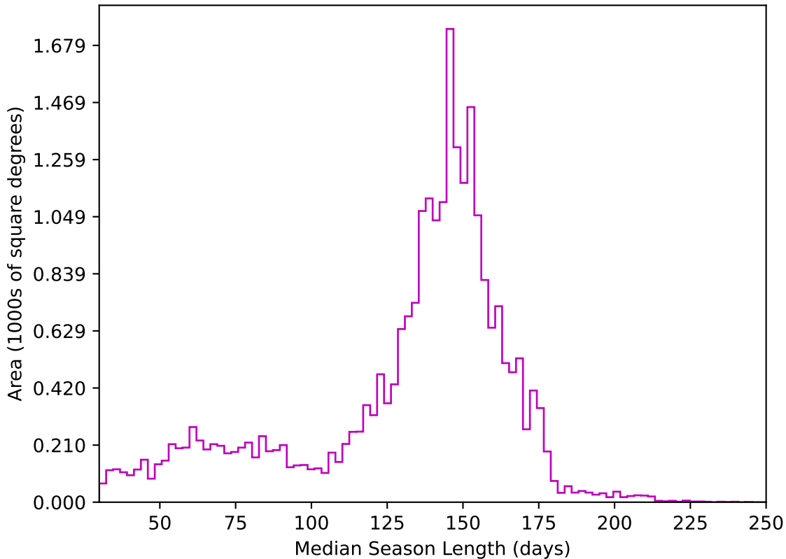
too_elab_r64_d3_griz_v3.4_10yrs All sky z band: Median Season Length
