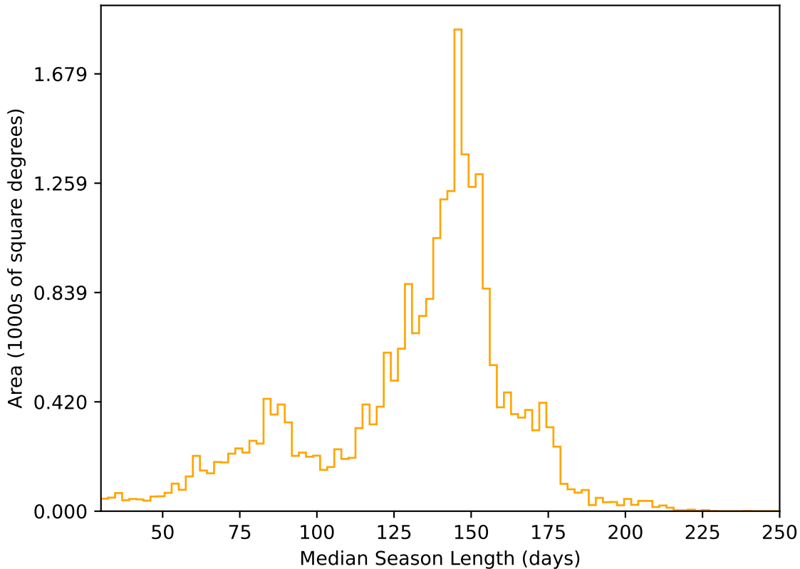
too_elab_r64_d3_griz_v3.4_10yrs All sky r band: Median Season Length
