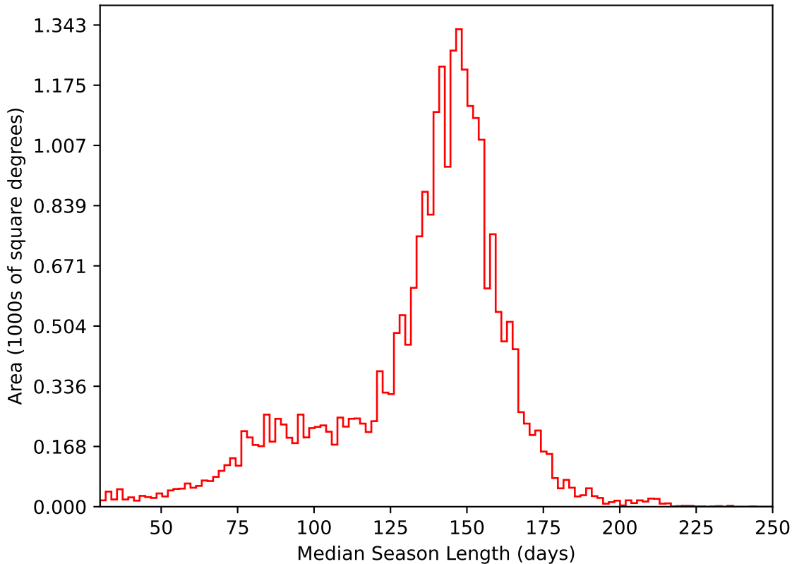
too_elab_r64_d3_griz_v3.4_10yrs All sky i band: Median Season Length
