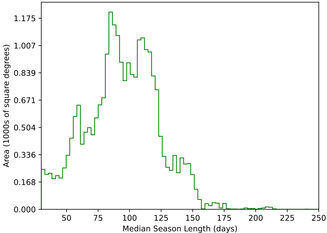
too_elab_r64_d3_griz_v3.4_10yrs All sky g band: Median Season Length
