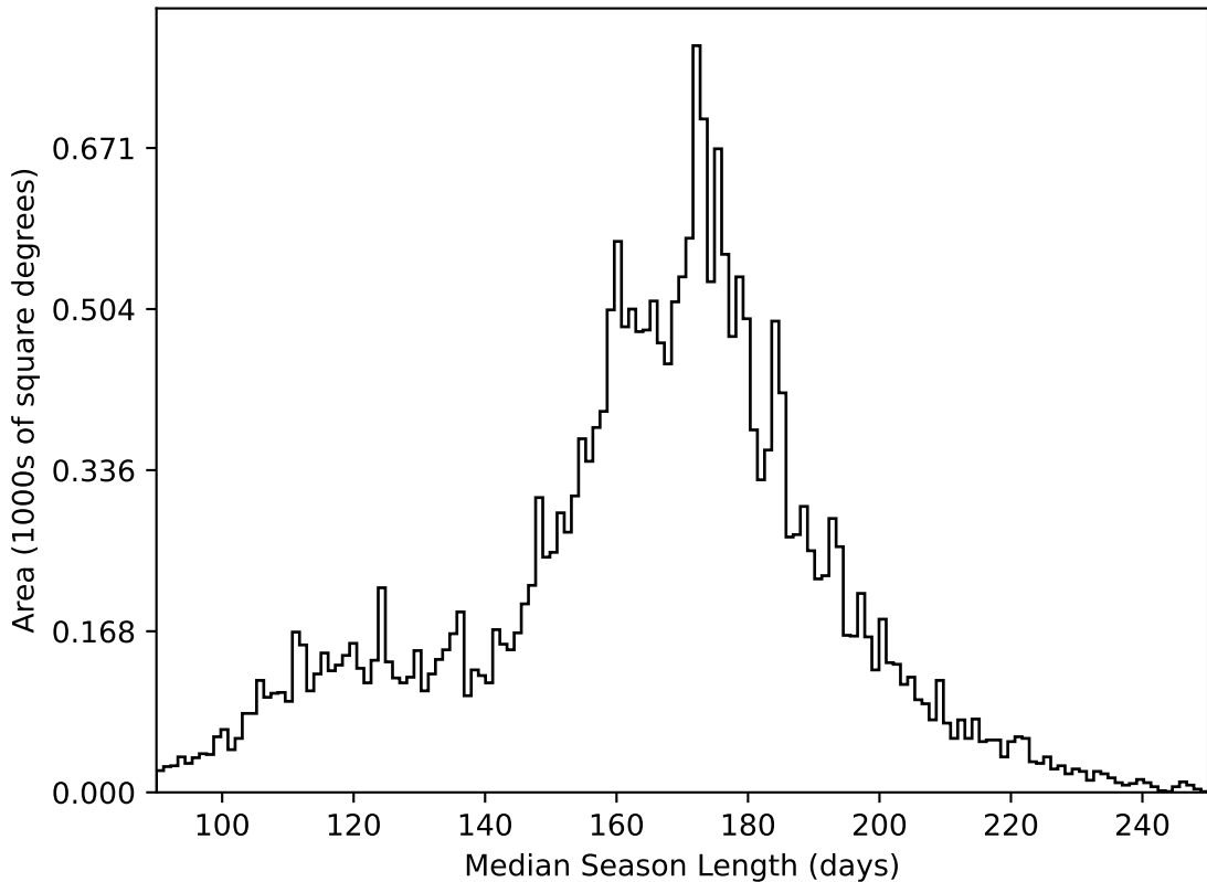
too_elab_r64_d3_griz_v3.4_10yrs All sky all bands: Median Season Length
