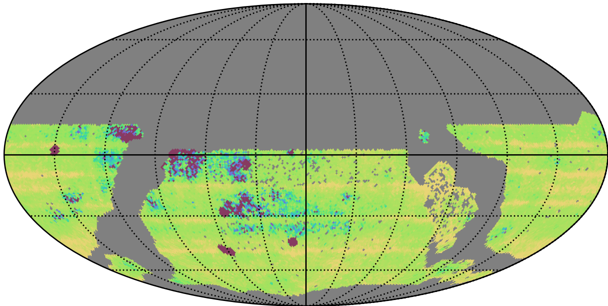
too_elab_r64_d3_griz_v3.4_10yrs WFD: Median Intra-Night Gap
