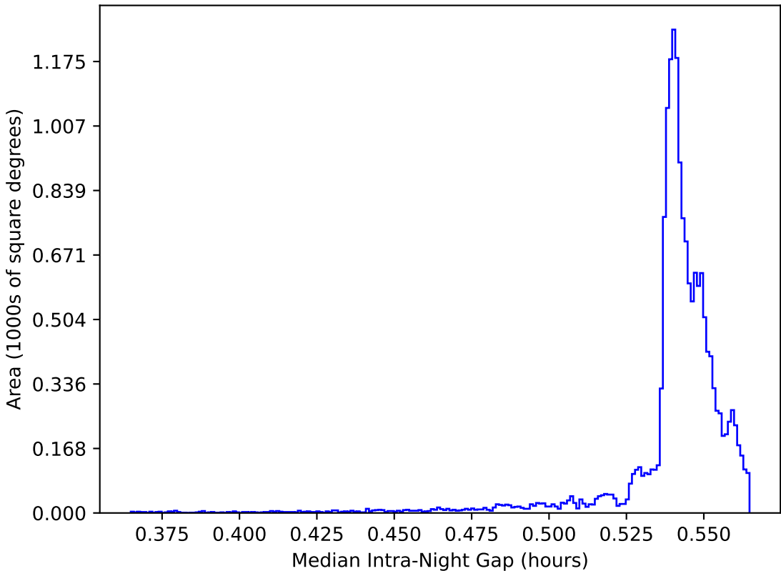
too_elab_r64_d3_griz_v3.4_10yrs WFD: Median Intra-Night Gap
