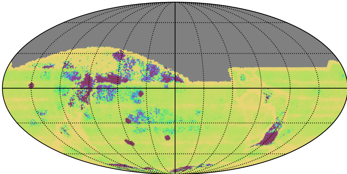
too_elab_r64_d3_griz_v3.4_10yrs All sky: Median Intra-Night Gap
