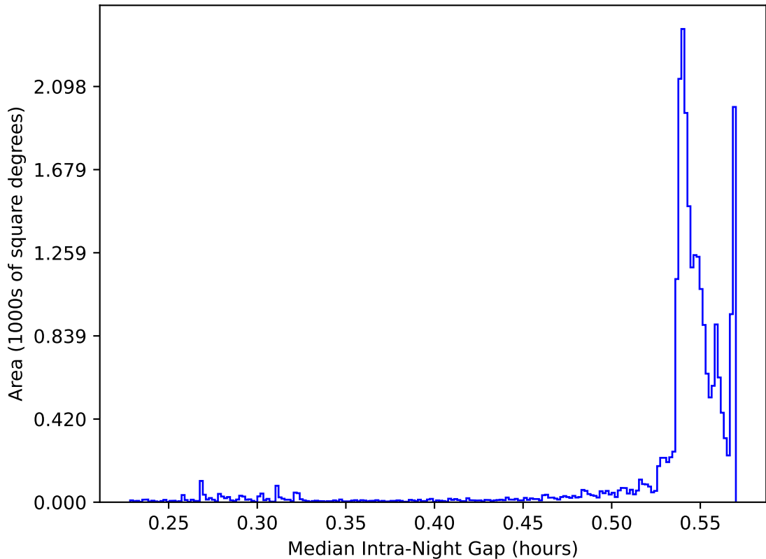
too_elab_r64_d3_griz_v3.4_10yrs All sky: Median Intra-Night Gap
