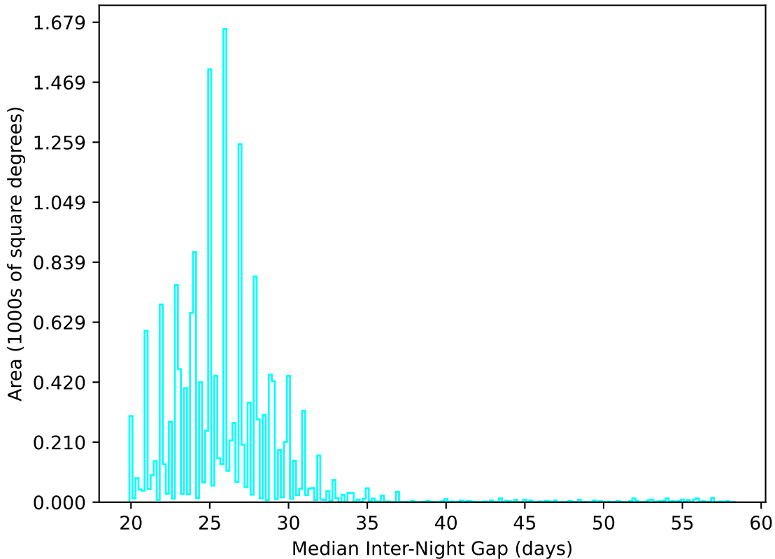
too_elab_r64_d3_griz_v3.4_10yrs WFD u band: Median Inter-Night Gap
