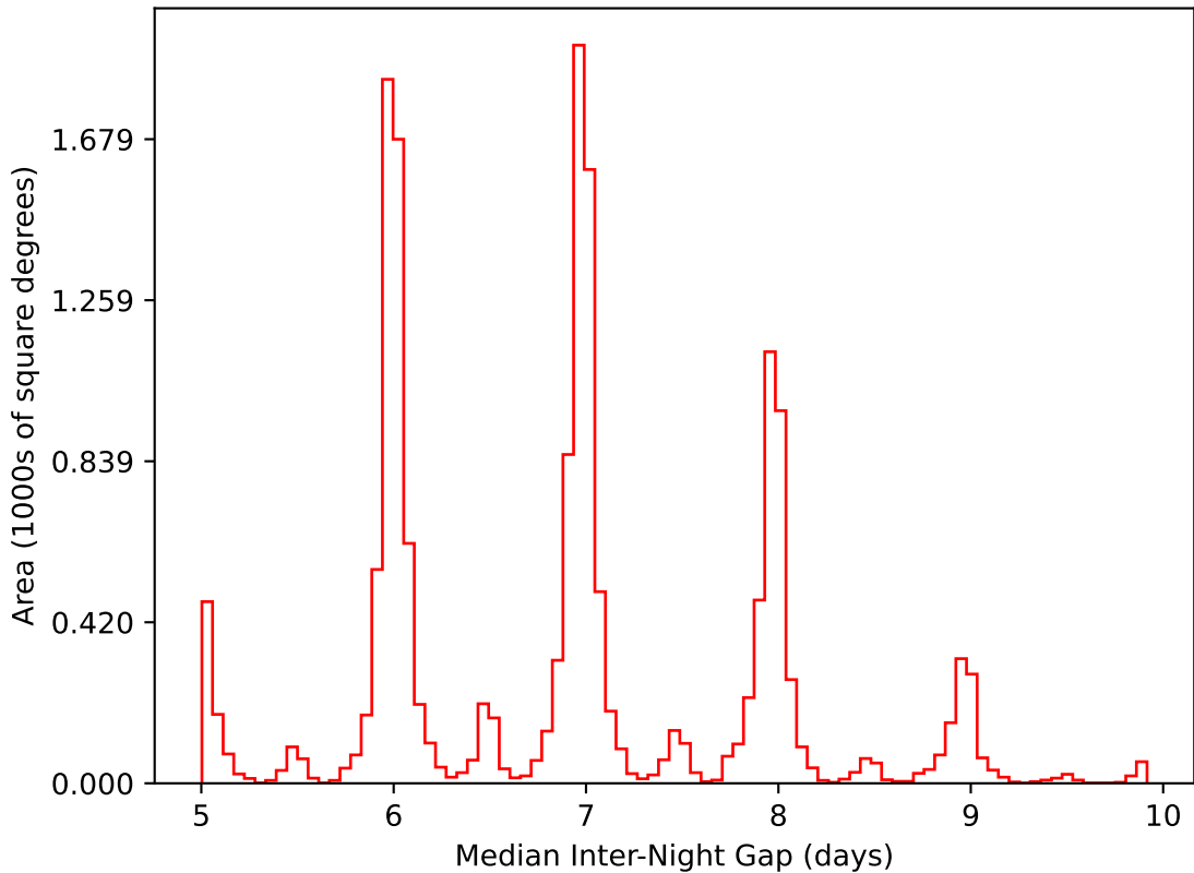
too_elab_r64_d3_griz_v3.4_10yrs WFD i band: Median Inter-Night Gap
