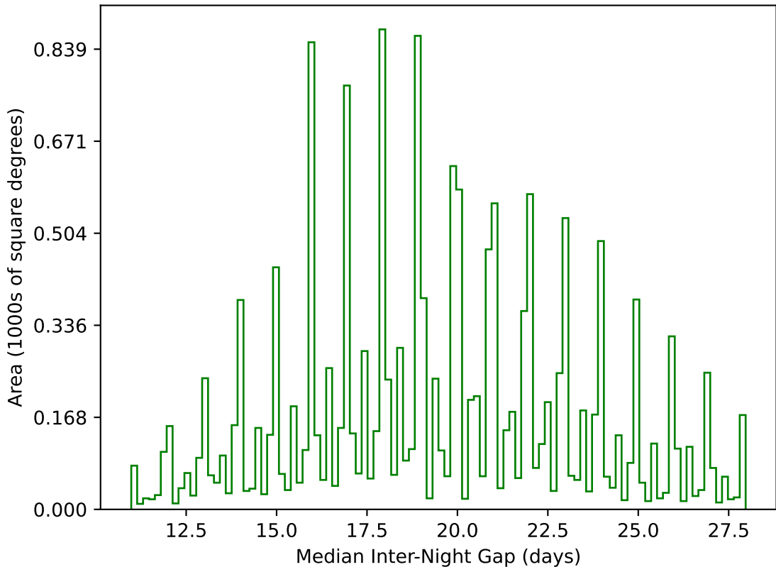
too_elab_r64_d3_griz_v3.4_10yrs WFD g band: Median Inter-Night Gap
