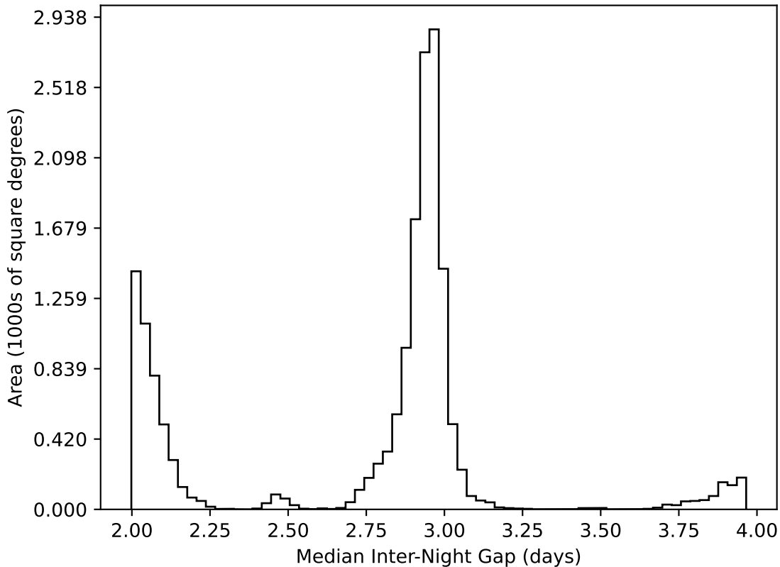
too_elab_r64_d3_griz_v3.4_10yrs WFD all bands: Median Inter-Night Gap
