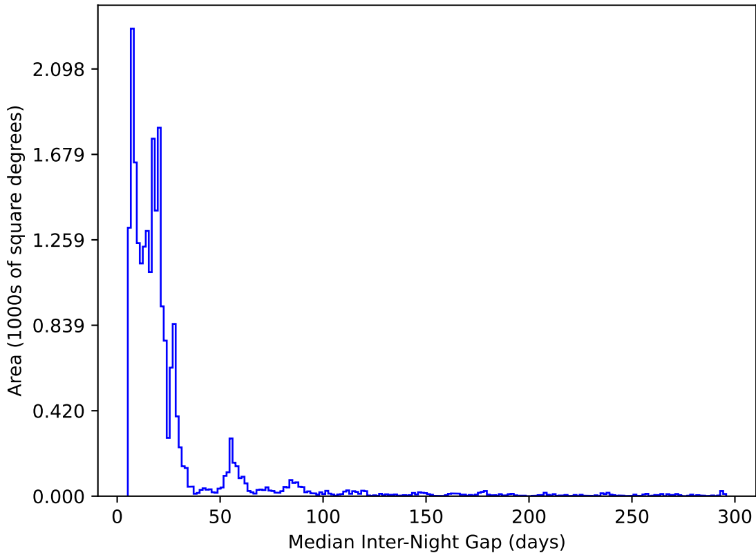
too_elab_r64_d3_griz_v3.4_10yrs All sky y band: Median Inter-Night Gap
