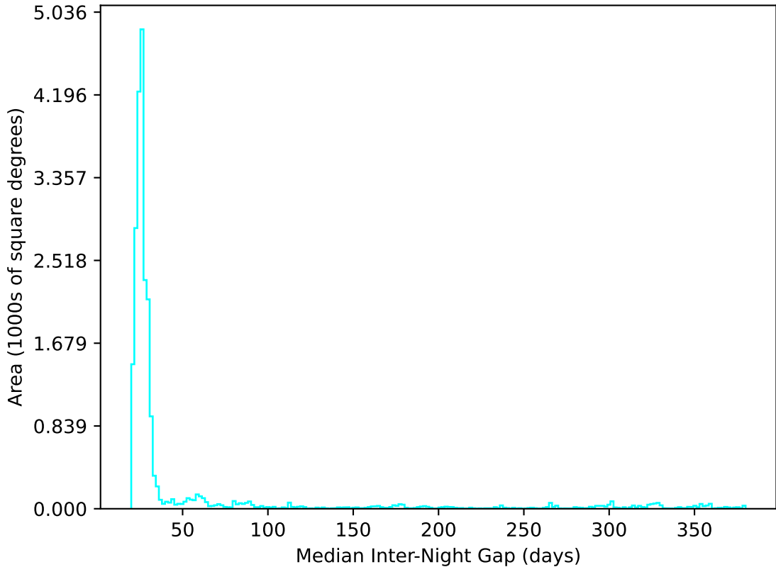
too_elab_r64_d3_griz_v3.4_10yrs All sky u band: Median Inter-Night Gap
