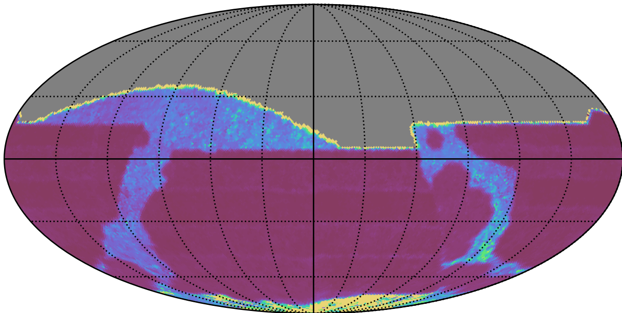
too_elab_r64_d3_griz_v3.4_10yrs All sky r band: Median Inter-Night Gap
