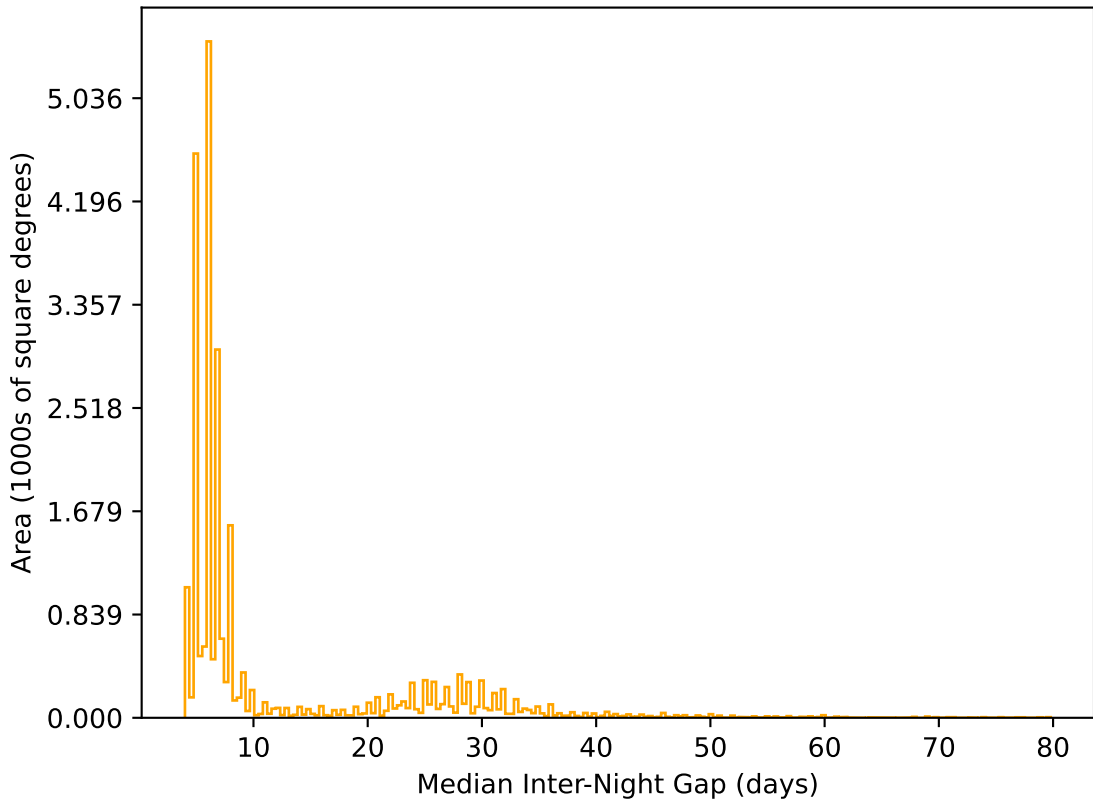
too_elab_r64_d3_griz_v3.4_10yrs All sky r band: Median Inter-Night Gap
