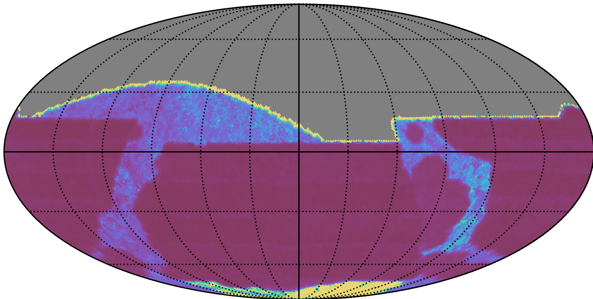
too_elab_r64_d3_griz_v3.4_10yrs All sky i band: Median Inter-Night Gap
