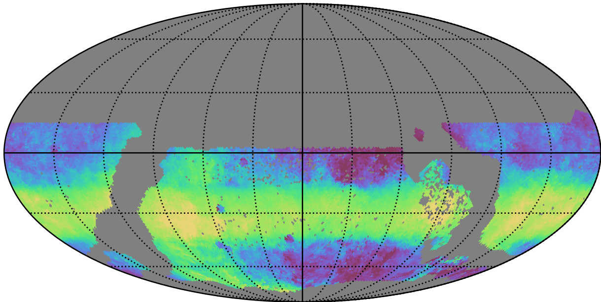
too_elab_r64_d3_griz_v3.4_10yrs WFD y band: Median HA
