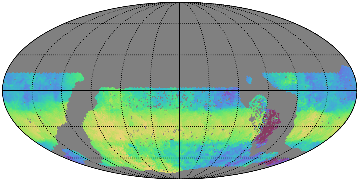
too_elab_r64_d3_griz_v3.4_10yrs WFD u band: Median HA
