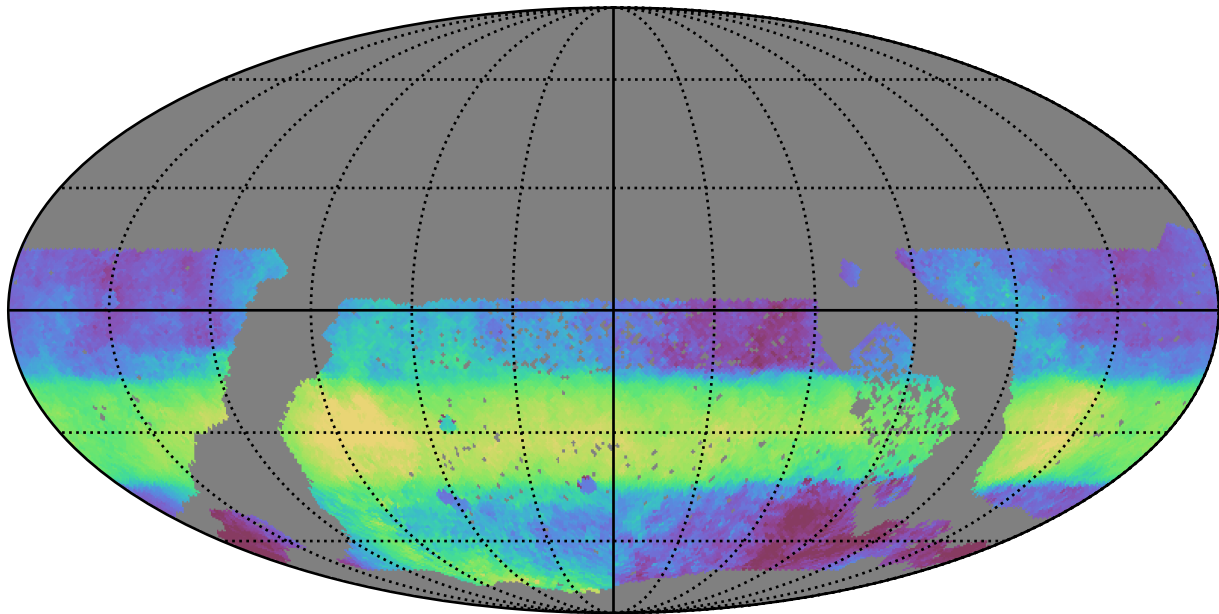
too_elab_r64_d3_griz_v3.4_10yrs WFD r band: Median HA
