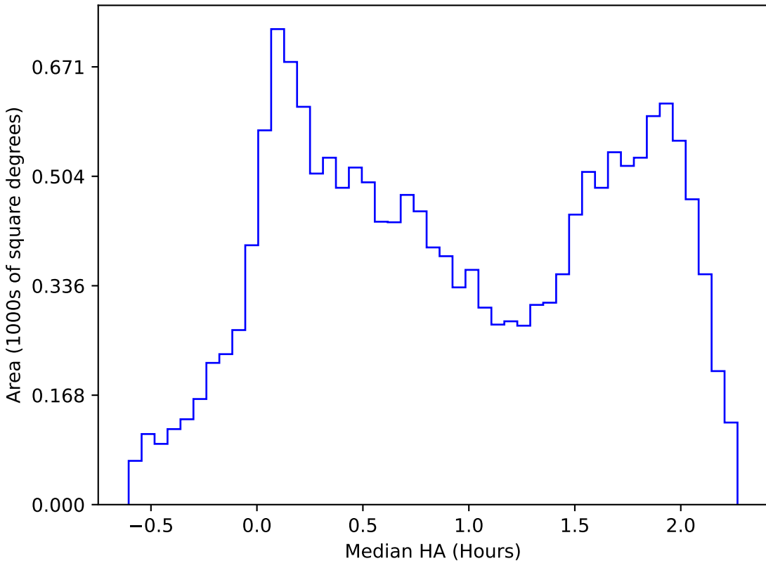
too_elab_r64_d3_griz_v3.4_10yrs WFD r band: Median HA
