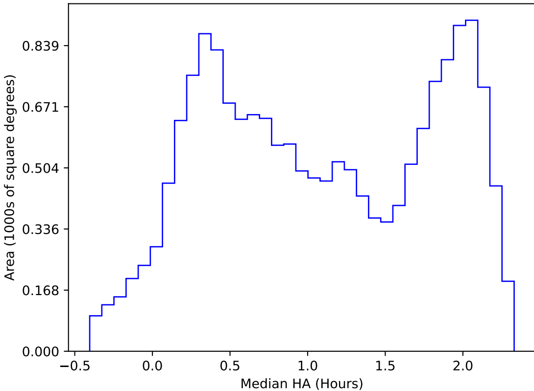
too_elab_r64_d3_griz_v3.4_10yrs WFD i band: Median HA
