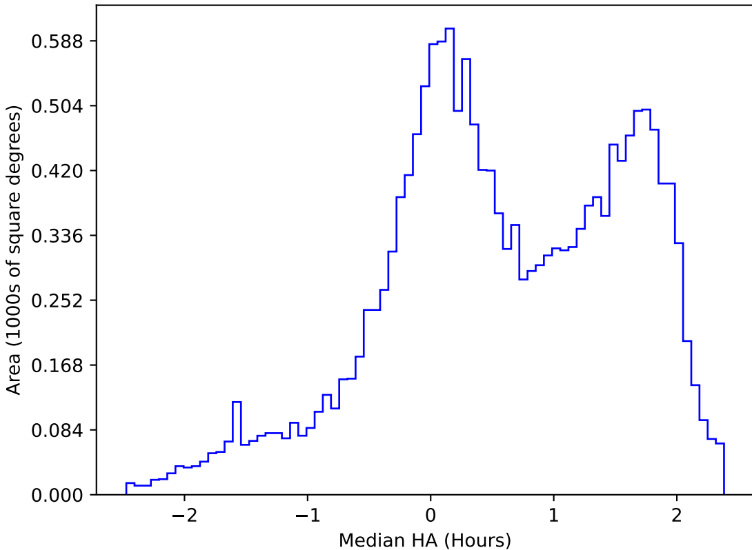
too_elab_r64_d3_griz_v3.4_10yrs WFD g band: Median HA
