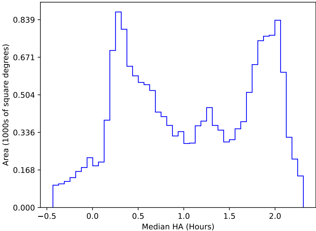
too_elab_r64_d3_griz_v3.4_10yrs WFD all bands: Median HA
