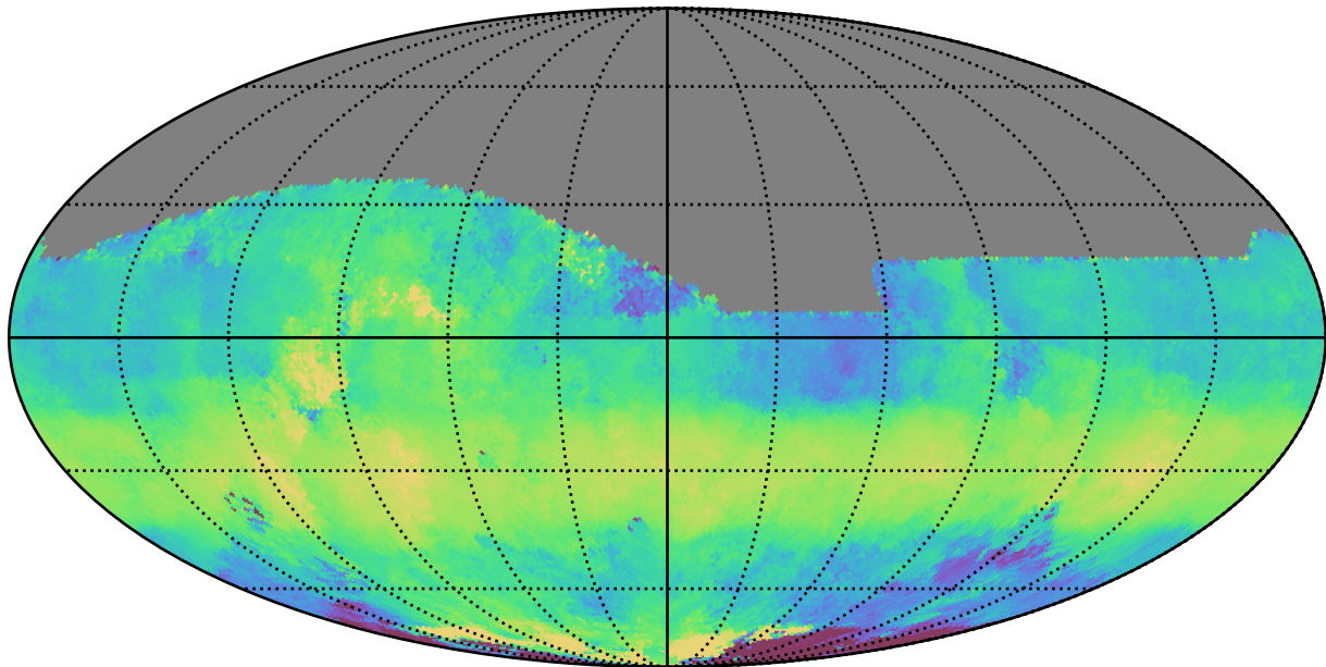
too_elab_r64_d3_griz_v3.4_10yrs All sky z band: Median HA
