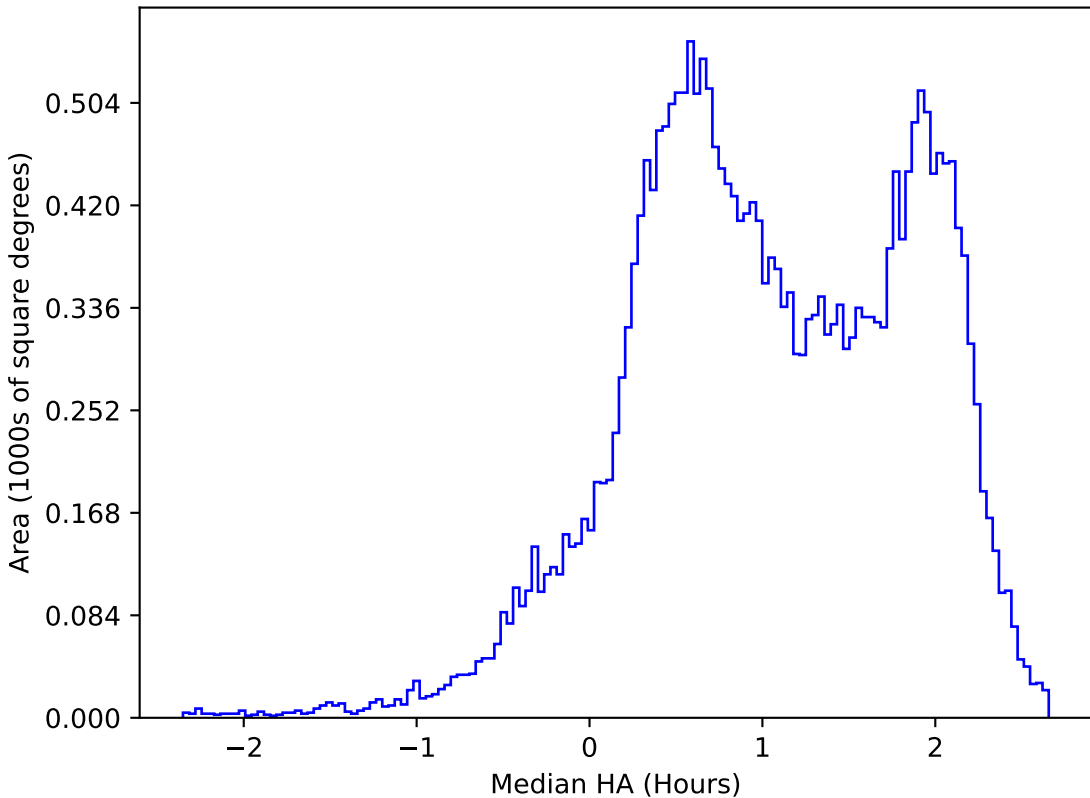
too_elab_r64_d3_griz_v3.4_10yrs All sky z band: Median HA
