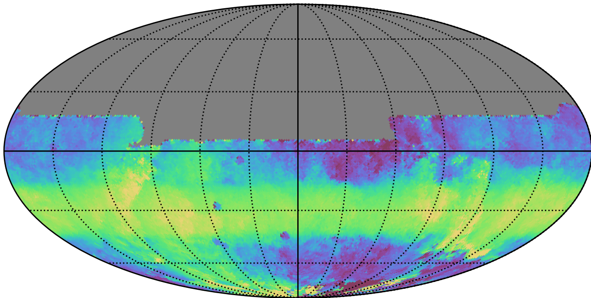
too_elab_r64_d3_griz_v3.4_10yrs All sky y band: Median HA
