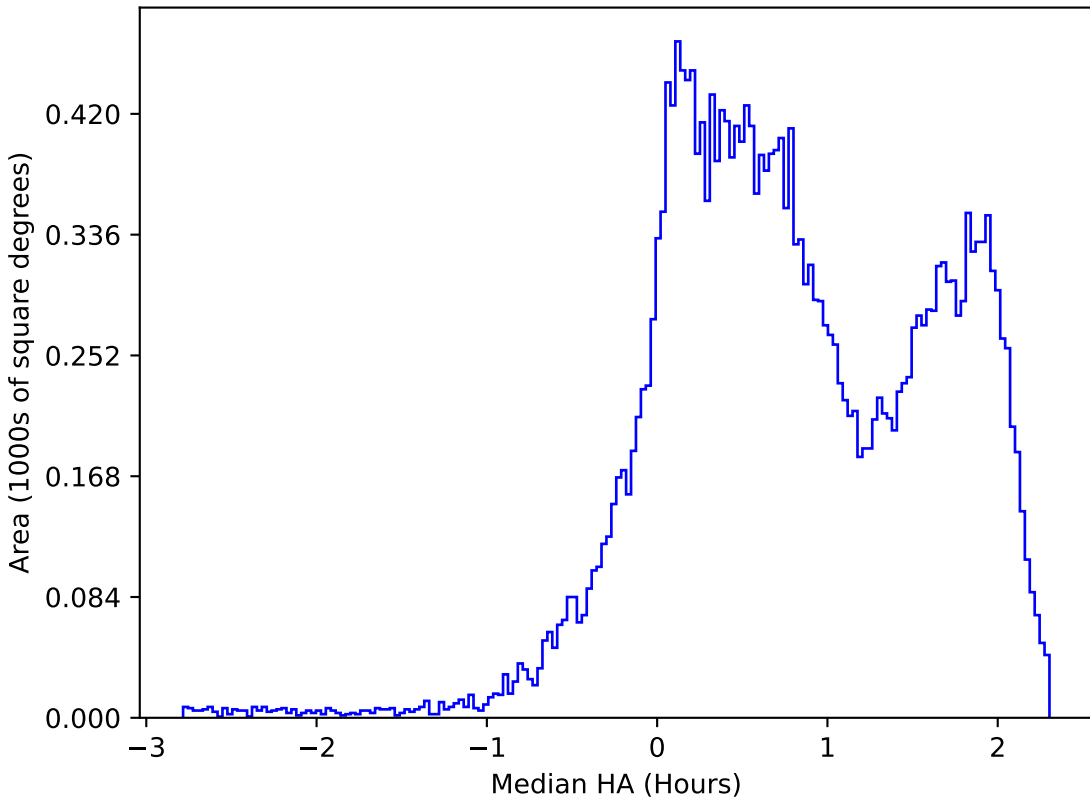
too_elab_r64_d3_griz_v3.4_10yrs All sky r band: Median HA
