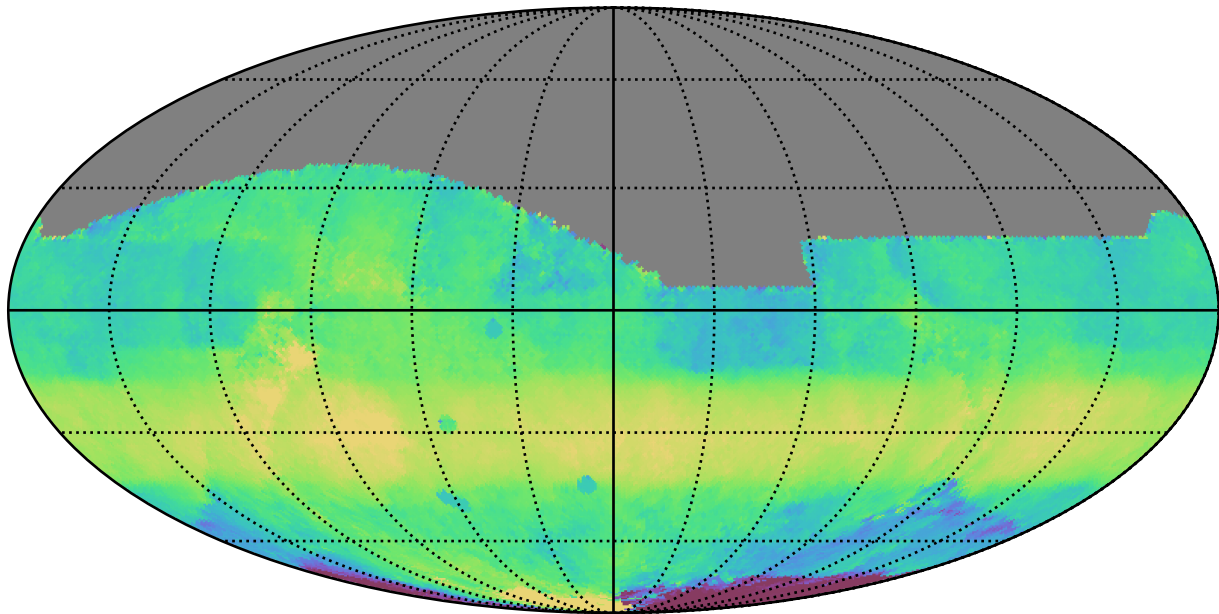
too_elab_r64_d3_griz_v3.4_10yrs All sky i band: Median HA
