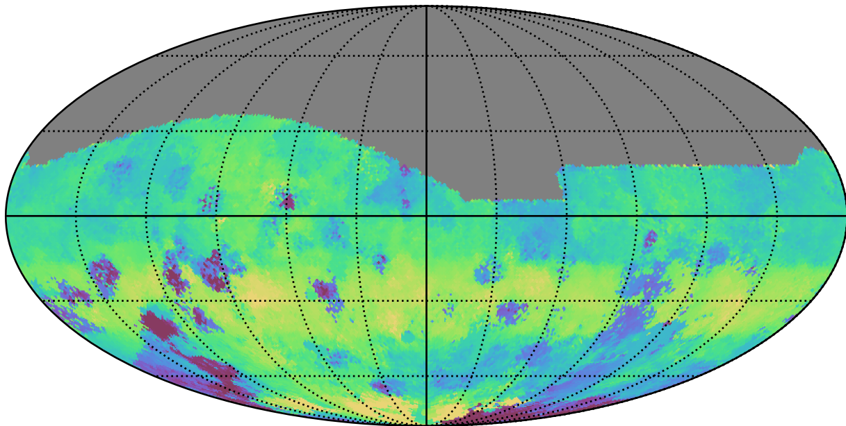
too_elab_r64_d3_griz_v3.4_10yrs All sky g band: Median HA
