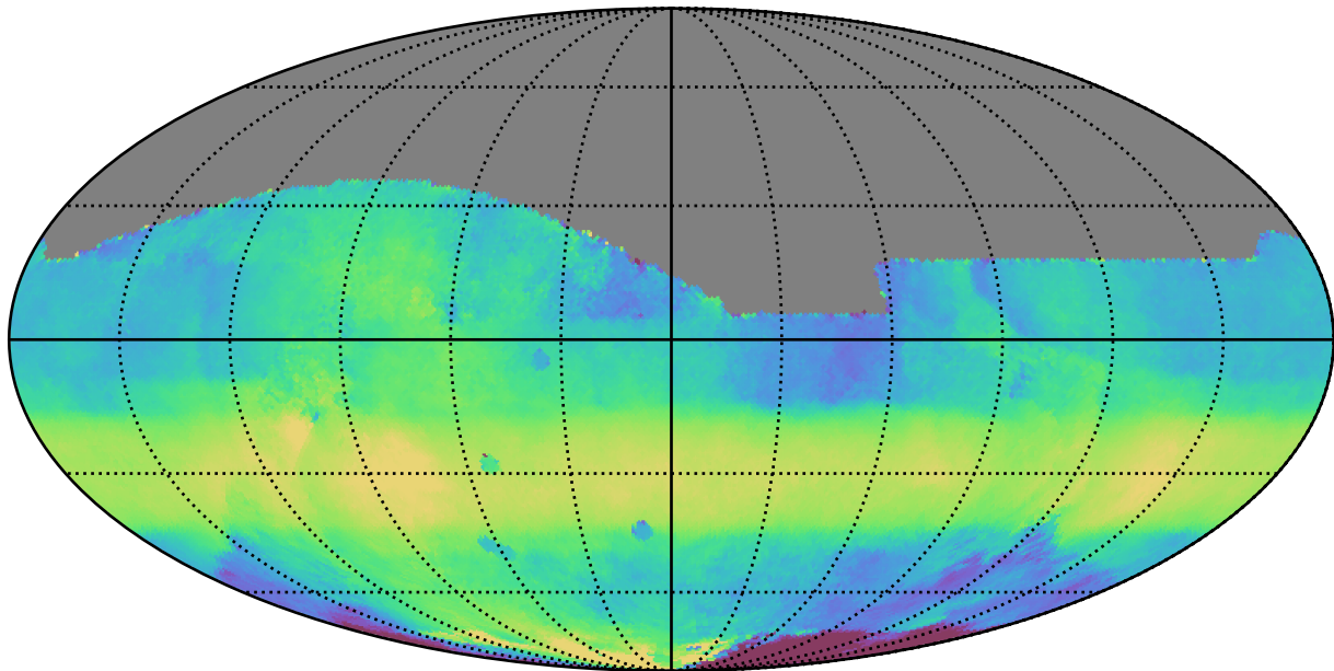
too_elab_r64_d3_griz_v3.4_10yrs All sky all bands: Median HA
