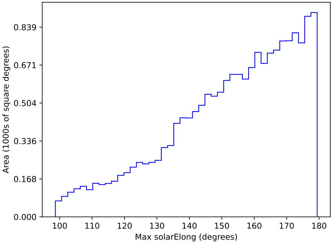
too_elab_r64_d3_griz_v3.4_10yrs WFD y band: Max solarElong
