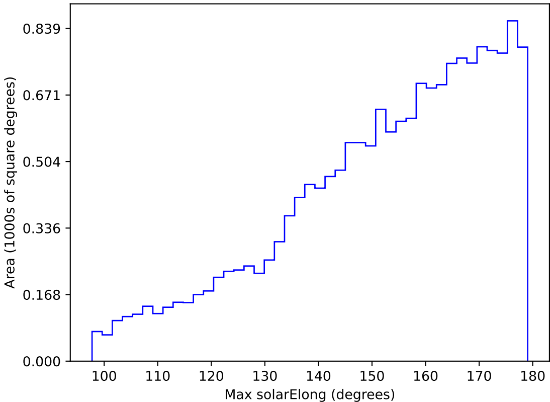
too_elab_r64_d3_griz_v3.4_10yrs WFD u band: Max solarElong
