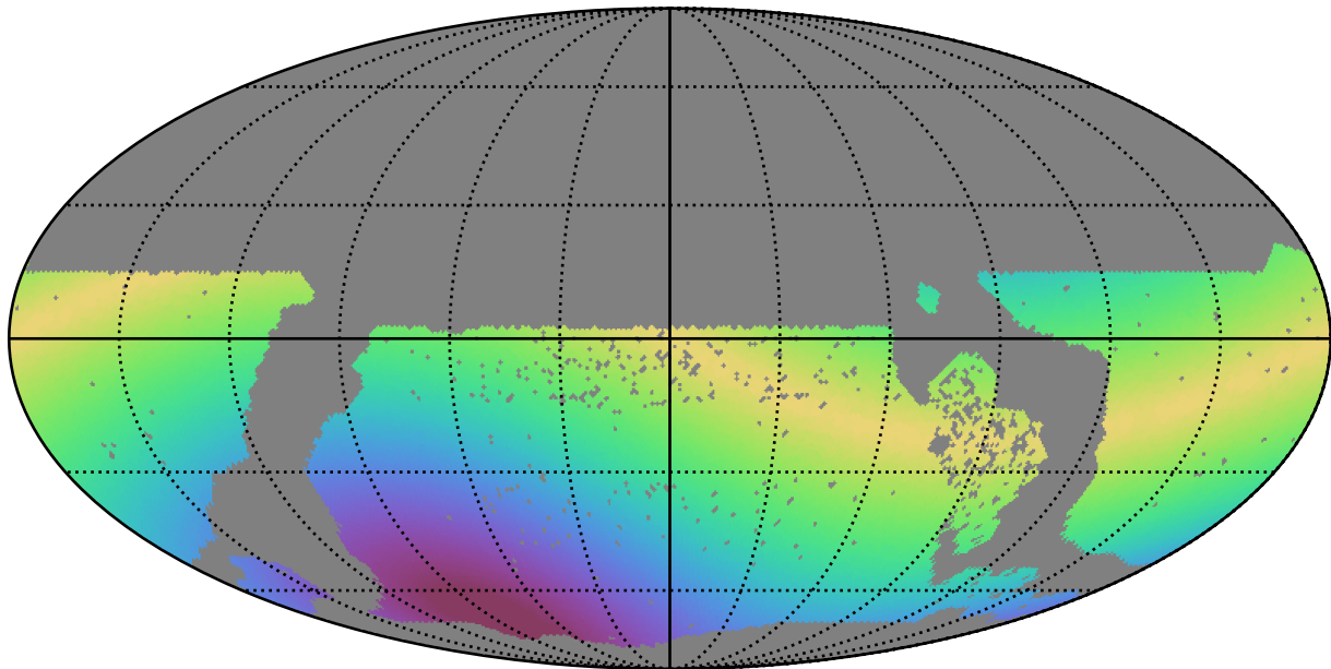
too_elab_r64_d3_griz_v3.4_10yrs WFD r band: Max solarElong
