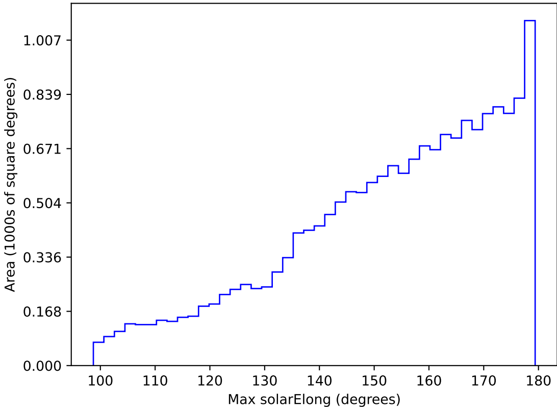
too_elab_r64_d3_griz_v3.4_10yrs WFD r band: Max solarElong
