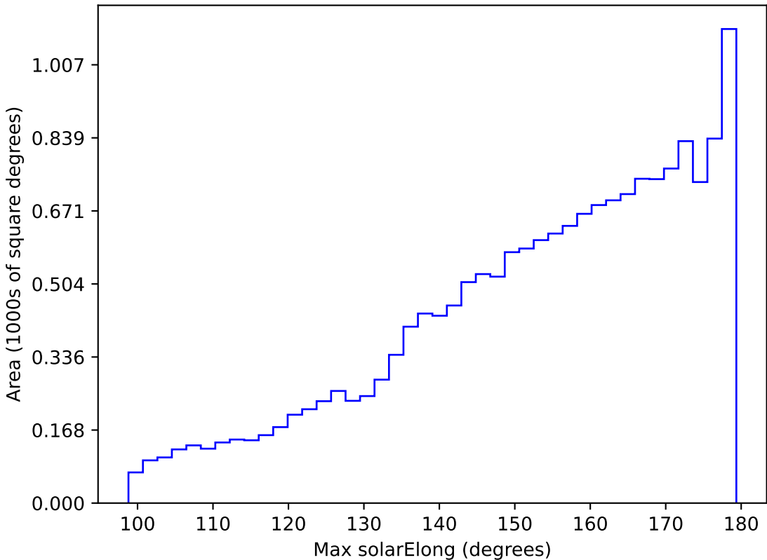
too_elab_r64_d3_griz_v3.4_10yrs WFD i band: Max solarElong
