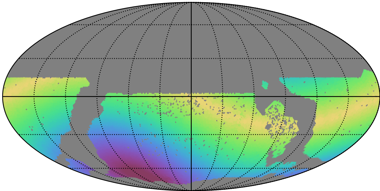
too_elab_r64_d3_griz_v3.4_10yrs WFD g band: Max solarElong
