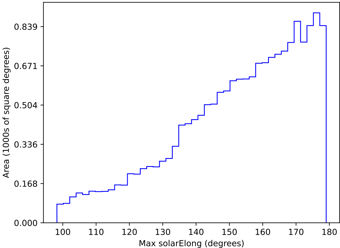
too_elab_r64_d3_griz_v3.4_10yrs WFD g band: Max solarElong
