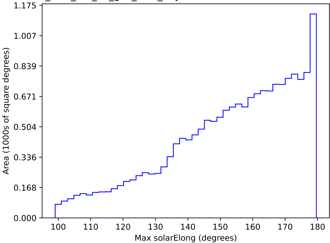
too_elab_r64_d3_griz_v3.4_10yrs WFD all bands: Max solarElong
