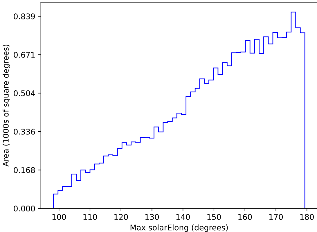
too_elab_r64_d3_griz_v3.4_10yrs All sky y band: Max solarElong
