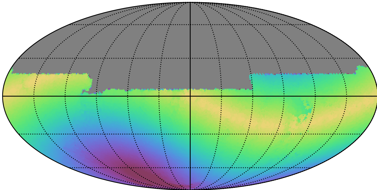
too_elab_r64_d3_griz_v3.4_10yrs All sky u band: Max solarElong
