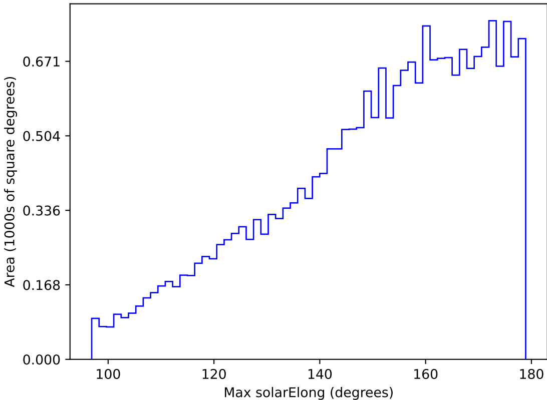
too_elab_r64_d3_griz_v3.4_10yrs All sky u band: Max solarElong
