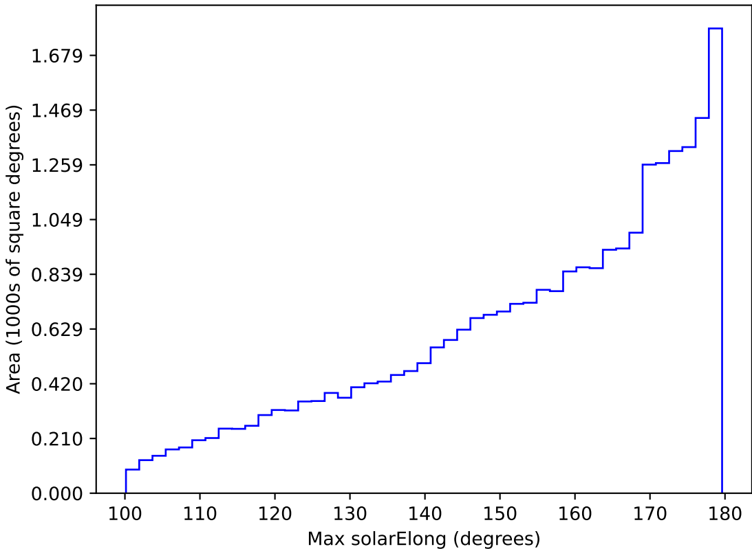
too_elab_r64_d3_griz_v3.4_10yrs All sky all bands: Max solarElong
