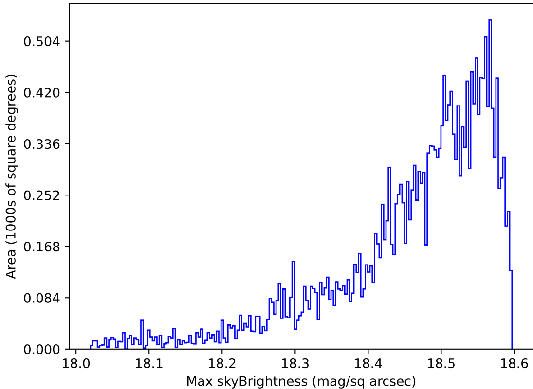
too_elab_r64_d3_griz_v3.4_10yrs Yr 1 y band: Max skyBrightness
