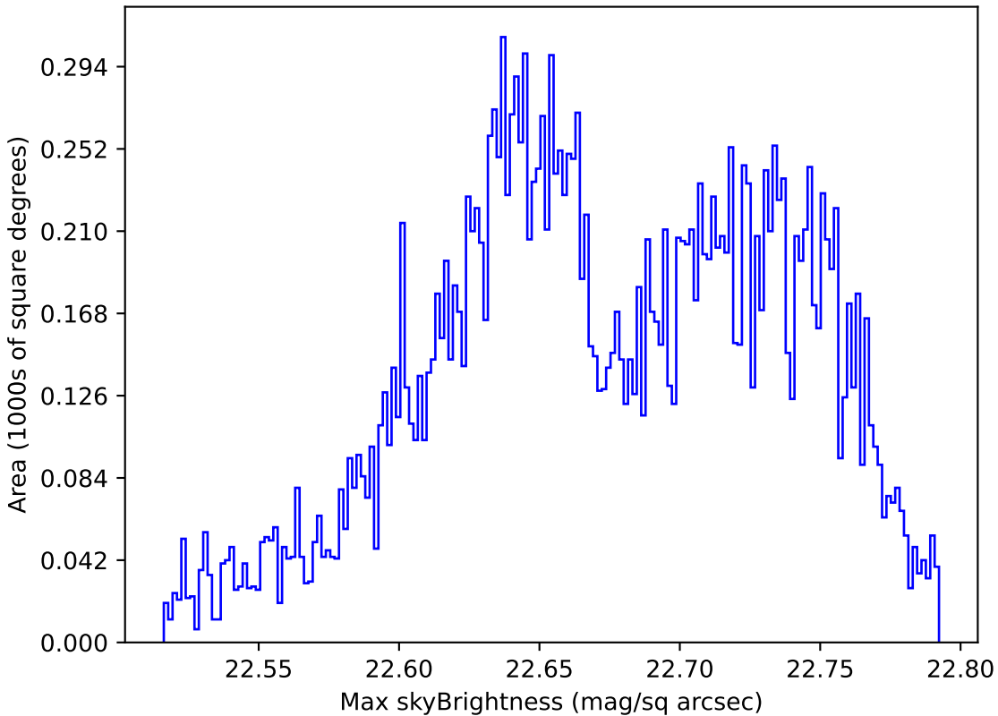
too_elab_r64_d3_griz_v3.4_10yrs Yr 1 u band: Max skyBrightness
